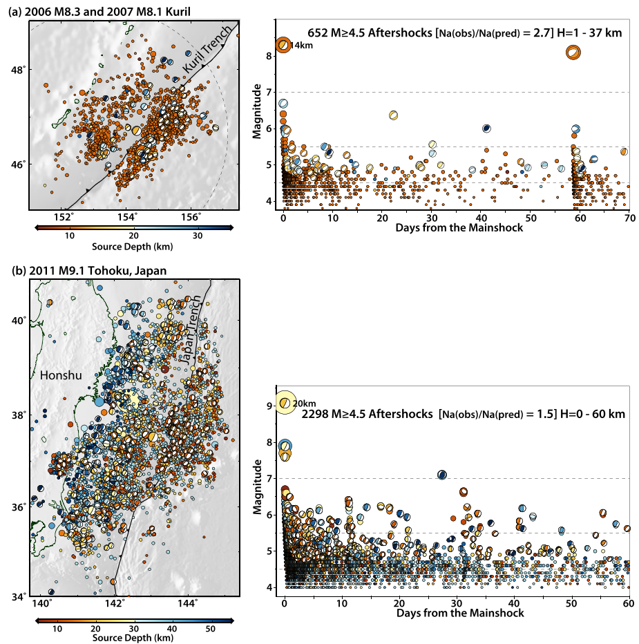
Figure 8. Complex earthquake sequences in old ocean lithosphere following great plate boundary thrust events in map view and as time series showing 70 or 60 day intervals of all seismicity from the USGS-NEIC catalog and all GCMT moment tensor solutions (both colored by source depth and scaled proportional to magnitude) within a two source dimension radius (dashed white lines are one source dimension radii) from each sequence mainshock for (a) 2006–2007 Kuril Islands Doublet and (b) 2011 Tohoku earthquake. The number of aftershocks, N_a (obs), with M \geq 4.5 within the indicated source depth ( H ) range over the 70 or 60 day window is indicated for each event, along with the ratio N_a (obs)/ N_a (pred) from Table 1. The GCMT centroid depth of the mainshock is shown next to the event focal mechanism.
