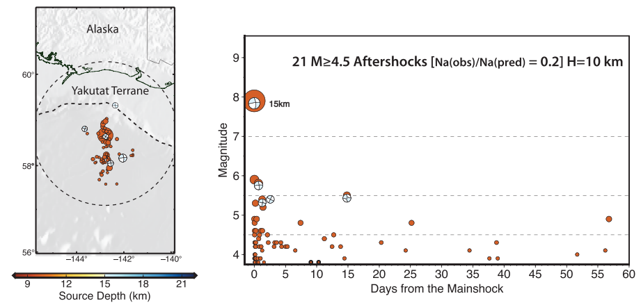
(c) 1988, Gulf of Alaska(3), M_w 7.8
