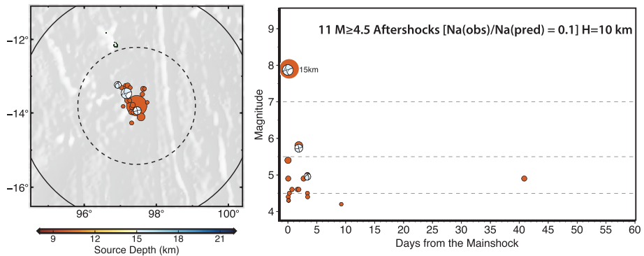
(c) 2016 Wharton, M_w 7.8
