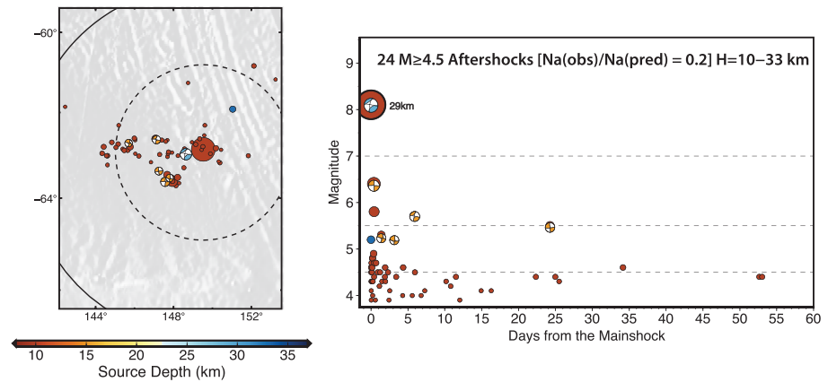
(b) 2000 Wharton, M_w 7.9
