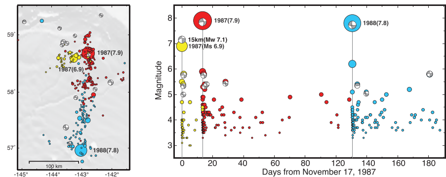
(b) 1987, Gulf of Alaska(2), M_w 7.9
