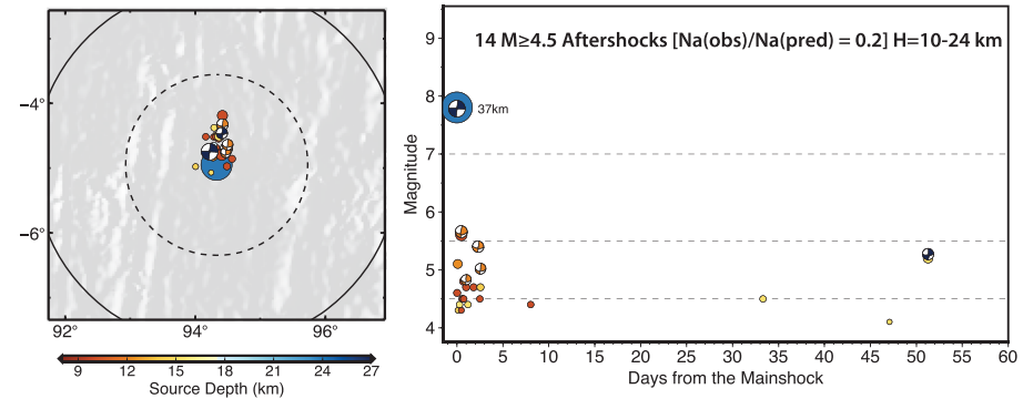
Figure 6. Modest complexity earthquake sequences with mainshock M_w \geq 7.8 in oceanic lithosphere well removed from subduction zones in map view and as time series showing 60 day intervals of all seismicity from the USGS-NEIC catalog and all GCMT moment tensor solutions (both colored by source depth and scaled proportional to magnitude) within a two source dimension radius (dashed white lines are one source dimension radii, and solid white lines are two source dimensions) from each sequence mainshock for (a) 1998 Balleny, (b) 2000 Wharton Basin, and (c) 2016 Wharton Basin (Table 1). The latter two events struck within the Indo-Australian plate further away from the subduction zone and outside the intraplate deformation zone where the 2012 sequence occurred. The number of aftershocks, N_a (obs), with M \geq 4.5 within the indicated source depth ( H ) range over the 60 day window is indicated for each event, along with the ratio of N_a (obs)/ N_a (pred) using the reference model discussed in the text. The GCMT centroid depth of the mainshock is shown next to the event focal mechanism.
