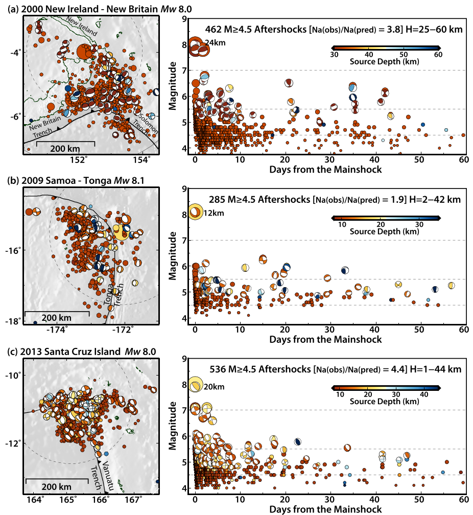
Figure 9. Complex earthquake sequences near sharp corners in subduction zones in map view and as time series showing 60 day intervals of all seismicity from the USGS-NEIC catalog and all GCMT moment tensor solutions (both colored by source depth and scaled proportional to magnitude) within a two source dimension radius (dashed white lines are one source dimension radii, and solid white lines are two source dimensions) from each sequence mainshock for (a) 2000 New Ireland-New Britain, (b) 2009 Samoa-Tonga, and (c) 2013 Solomon-Santa Cruz Island. The number of aftershocks, N_a (obs), with M \geq 4.5 within the indicated source depth ( H ) range over the 60 day window is indicated for each event, along with the ratio N_a (obs)/ N_a (pred) from Table 1. The GCMT centroid depth of the mainshock is shown next to the event focal mechanism.
