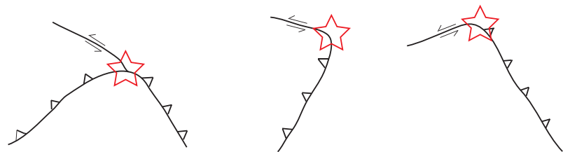
Figure 11. Tectonic scenarios giving rise to complex intraplate sequences in oceanic lithosphere. (a) Laterally varying stress along subduction zones arising from convergence of oceanic plateaus or continental material adjacent to oceanic convergent zone that have strong slab pull and large earthquake cycles give rise to complex strike-slip sequences seaward of the outer rise (Figures 4b–4d and 5) or complex obliquely trending normal fault sequences near the trench (Figure 4a) and less complex strike-slip sequences further from the boundary (Figure 6). (b) Slab bending stresses driven by slab pull, modulated by earthquake cycle stresses activate multiple normal-fault systems in the outer trench slope and outer rise (Figure 7). (c) Sharp corners in subduction zones associated with slab draping (left), lithospheric tearing (middle), and slab edges (right), produce complex sequences with interplate and intraplate faulting, which can extend into old oceanic lithosphere (Figure 8).
