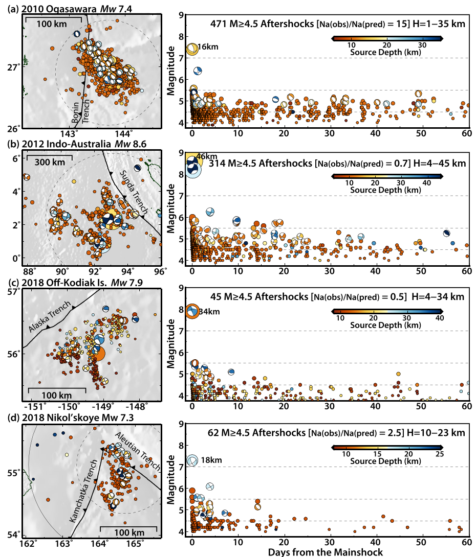
Figure 4. Complex earthquake sequences in oceanic lithosphere seaward of trenches showing 60 day intervals of all seismicity from the USGS-NEIC catalog and all GCMT moment tensor solutions (both colored by source depth and scaled proportional to magnitude) within a two source dimension radius (dashed black lines are one source dimension radii, solid black lines are two source dimensions) from each mainshock for: (a) 2010 Ogasawara (Bonin), (b) 2012 Indo-Australia, (c) 2018 Off-Kodiak Island, and (d) 2018 Nikol'skoye. The number of aftershocks, Na (obs), with M \geq 4.5 within the indicated source depth ( H ) range over the 60 day window is indicated for each event, along with the ratio Na (obs)/ Na (pred) from Table 1. The GCMT centroid depth of the mainshock is shown next to the event focal mechanism.
