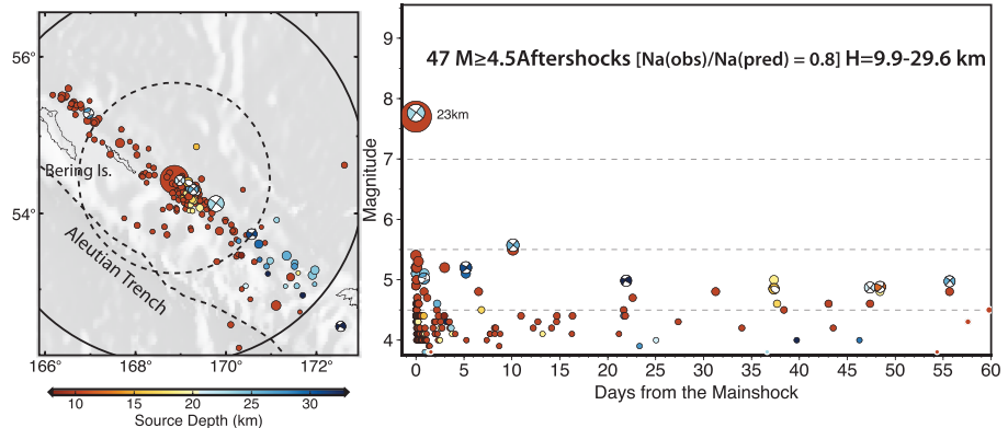
Figure 10. Large oceanic strike-slip earthquake sequences in oceanic lithosphere in map view and as time series showing 60 day intervals of all seismicity from the USGS-NEIC catalog and all GCMT moment tensor solutions (both colored by source depth and scaled proportional to magnitude) within a two source dimension radius (dashed white lines are one source dimension radii, and solid white lines are two source dimensions) from each sequence mainshock for (a) 2013 Craig, Alaska, and (b) 2017 Komandorsky Islands (Western Aleutians) along the Bering Fracture Zone. The number of aftershocks, N_a (obs), with M \geq 4.5 within the indicated source depth ( H ) range over the 60 day window is indicated for each event, along with the ratio of N_a (obs)/ N_a (pred) using the reference model discussed in the text. The GCMT centroid depth of the mainshock is shown next to the event focal mechanism.
