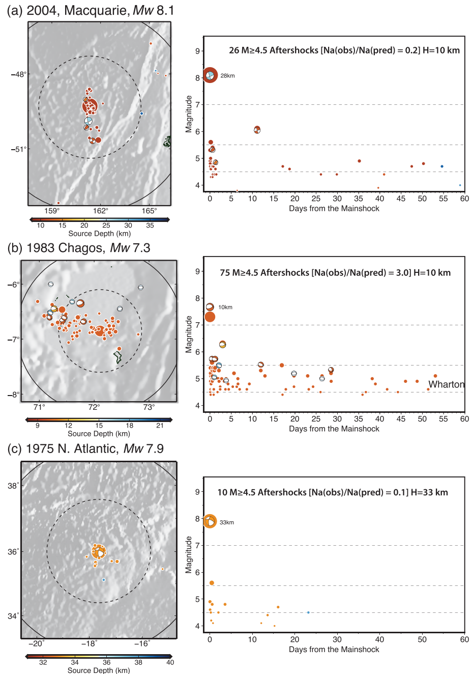
Figure 7. Additional modest complexity earthquake sequences with mainshock M_W \geq 7.3 in oceanic lithosphere well removed from subduction zones in map view and as time series showing 60day intervals of all seismicity from the USGS-NEIC catalog and all GCMT moment tensor solutions (both colored by source depth and scaled proportional to magnitude) within a two source dimension radius (dashed white lines are one source dimension radii, and solid white lines are two source dimensions) from each sequence mainshock for (a) 2004 Macquarie; (b) 1983 Chagos, and (c) 1975 North Atlantic (Table 1). The focal mechanism for the 1975 event is from Lynnes and Ruff (1985). The number of aftershocks, N_a (obs), with M \geq 4.5 within the indicated source depth ( H ) range over the 60 day window is indicated for each event, along with the ratio of N_a (obs)/ N_a (pred) using the reference model discussed in the text. The GCMT centroid depth of the mainshock is shown next to the event focal mechanism.
