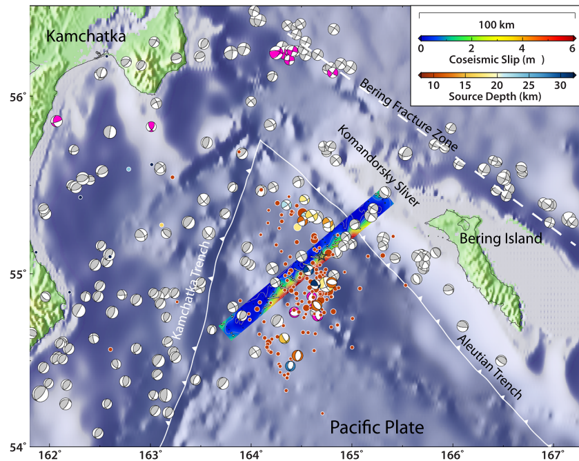
Figure 3. Map showing the 2018 Nikol'skoye M_W 7.4 mainshock finite-slip model from Figure S8 along with aftershocks in the first 60 days after the event from the USGS-NEIC catalog (circles with radius proportional to magnitude) and GCMT focal mechanisms plotted at the centroid locations, colored by centroid depth, and scaled by M_W . Focal mechanisms colored in gray and magenta are for the time periods of 1976 to 2018 before the mainshock and 2018 to 2019 after the mainshock, respectively. The Aleutian Trench has no convergence in this region, with the Komandorsky Sliver moving parallel to the Pacific plate motion with right-lateral shearing on the Bering Fracture Zone.
