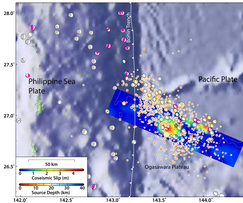
Figure 2. Map showing the 2010 Ogasawara M_W 7.4 mainshock finite-slip model from Figure S2 (the star indicates the mainshock epicenter) along with aftershocks in the first 60 days after the event from the USGS-NEIC catalog (circles colored by source depth and with radius proportional to magnitude) and GCMT focal mechanisms plotted at the centroid locations, colored by centroid depth and scaled by M_W . Focal mechanisms colored in gray and magenta are for the time periods of 1976 to 2010 before the mainshock and 2011 to 2019 after the mainshock, respectively. The background bathymetry indicates the position of the Bonin trench trending north-south near longitude 143.2°, approximated by the white saw-toothed curve.
