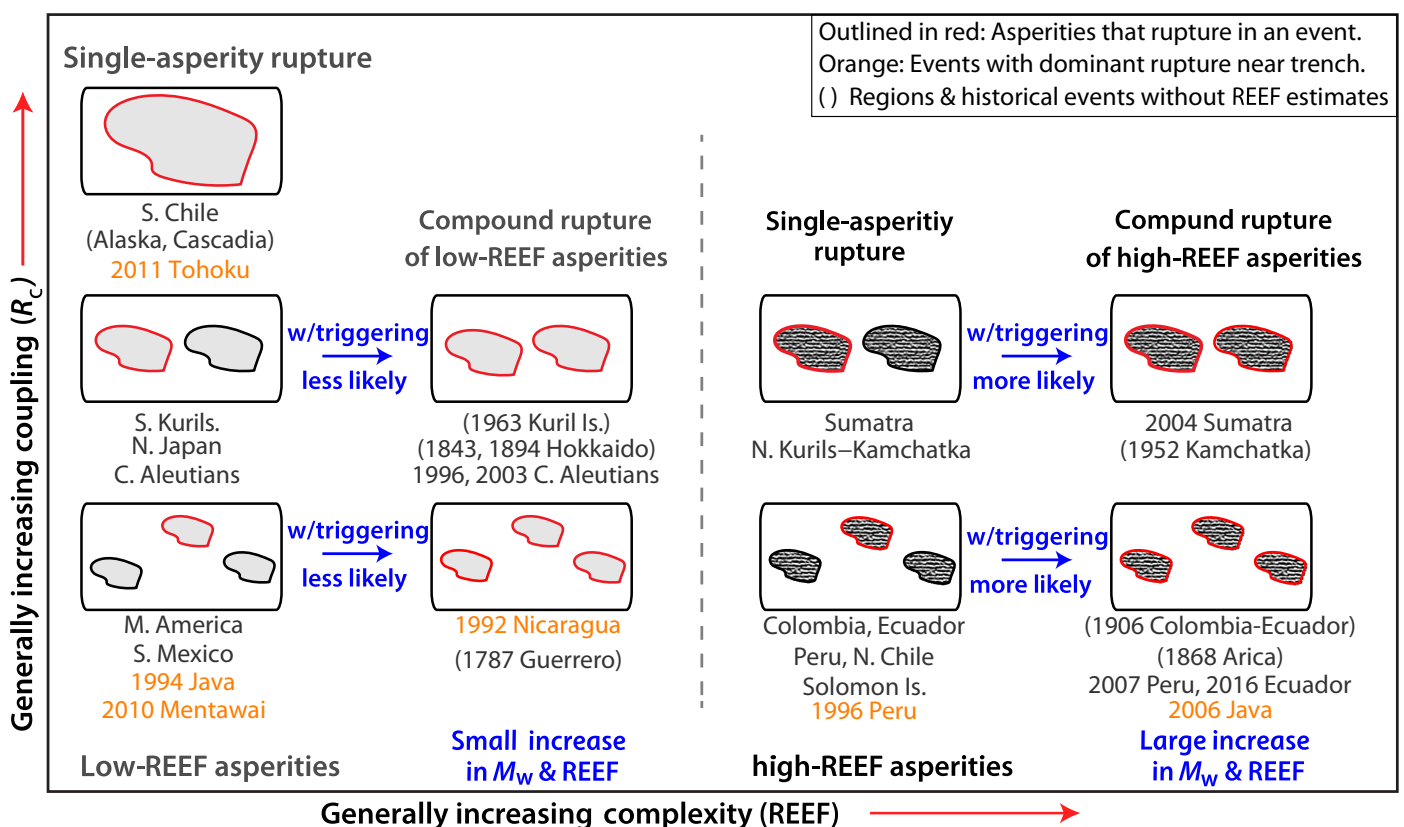
Fig. 5. Schematic categorization of ruptures associated with varying REEF and R_C values. Regions with slip patches of varying size and spacing, indicating variable fraction of asperity area R_C , can have ruptures that either produce low REEF values (left side, with light shading indicating smooth, simple rupture) or produce high REEF values (right side, with dark shading indicating rough, complex ruptures). Individual slip patches may fail or they may trigger additional slip patches, which increases REEF and earthquake magnitude overall within either category. Rough regions are more likely to have compound rupture due to triggering with relatively larger increases in magnitude and REEF. Below each schematic, specific subduction zones and events in that category are listed. Earthquakes labeled in orange are dominated by the near-trench rupture. Labeled regions or earthquakes in parentheses lack REEF measurements but are assigned to categories based on qualitative rupture attributes. Kuril Is., Kuril Islands; Solomon Is., Solomon Islands.
