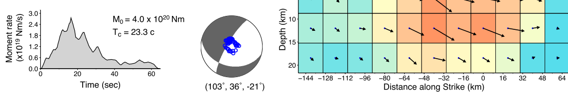
Fig. 7. Finite-fault slip models from inversion of teleseismic body waves (P and SH) for (a) November, 17, 2013, and (b) August 4, 2003 Scotia earthquakes. The slip distribution on the fault plane is shown with the arrows indicating average rake of each subfault, and slip magnitude being color-coded. Three contiguous fault segments with different geometries are used for the 2013 event with relative locations shown in Fig. 9(a). Rupture expansion velocity of 2.5 km/s is used for both events. The moment-rate functions, seismic moments, centroid time shift ( T_c ) and the average focal mechanism for each fault segment are shown, with lower hemisphere equal area projections indicating the positions sampled by teleseismic P waves used in the inversions. Observed and synthetic waveform comparisons are shown in the supplementary Fig. S6 and Fig. S7.
